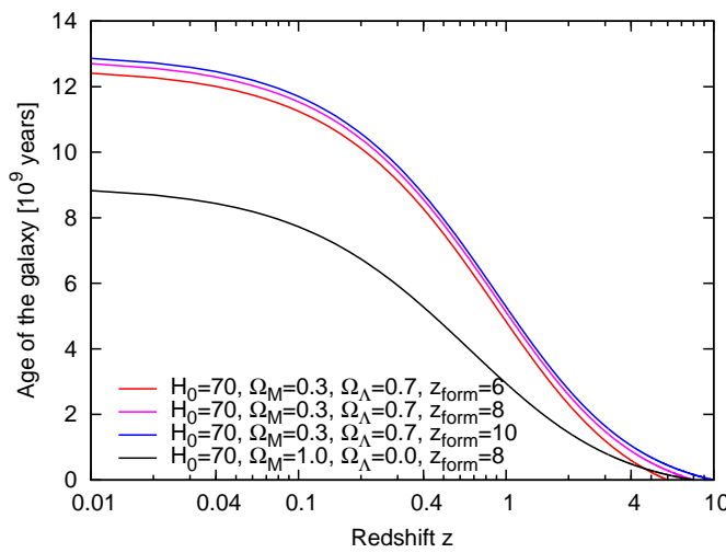
Figure C.11: Relation between galaxy age and redshift for different cosmological parameters and in particular varying formation redshifts.
