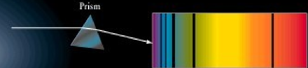
Absorption line spectrum
