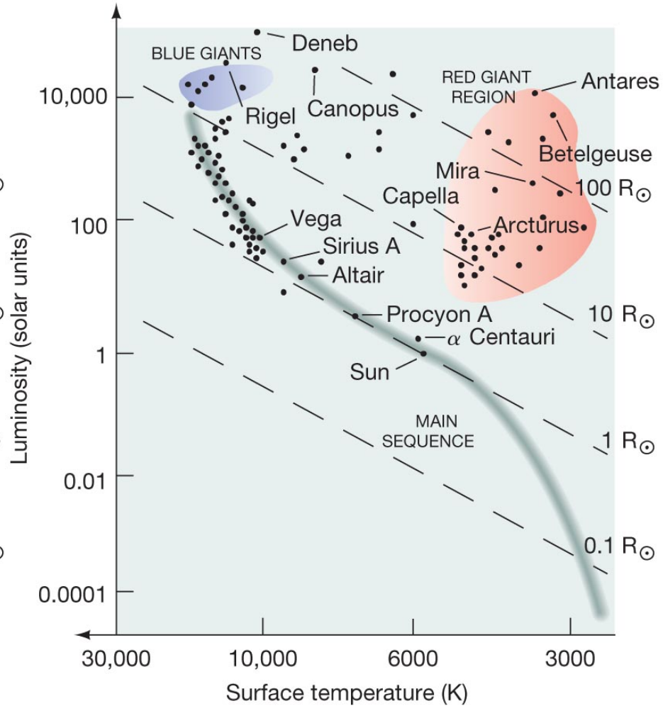
H-R diagram for bright stars
