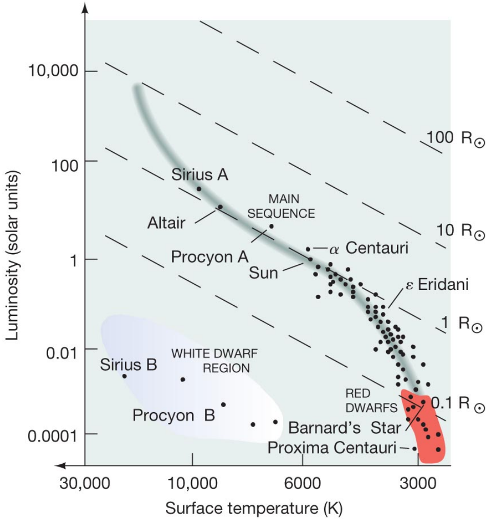
H-R diagram for nearby stars
