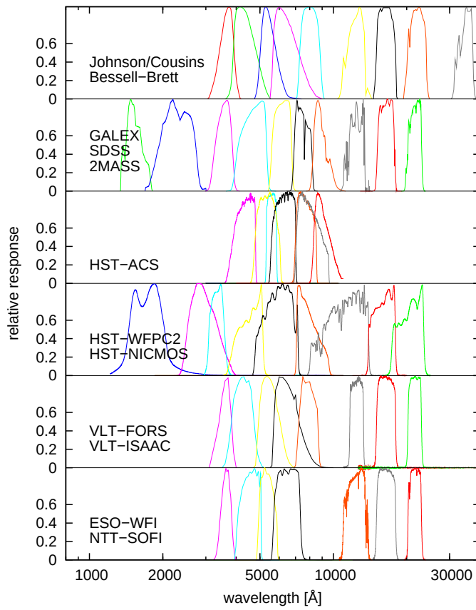
Figure C.15: Selection of the filters currently offered by GALEV, ranging from the far-UV to near-infrared.
