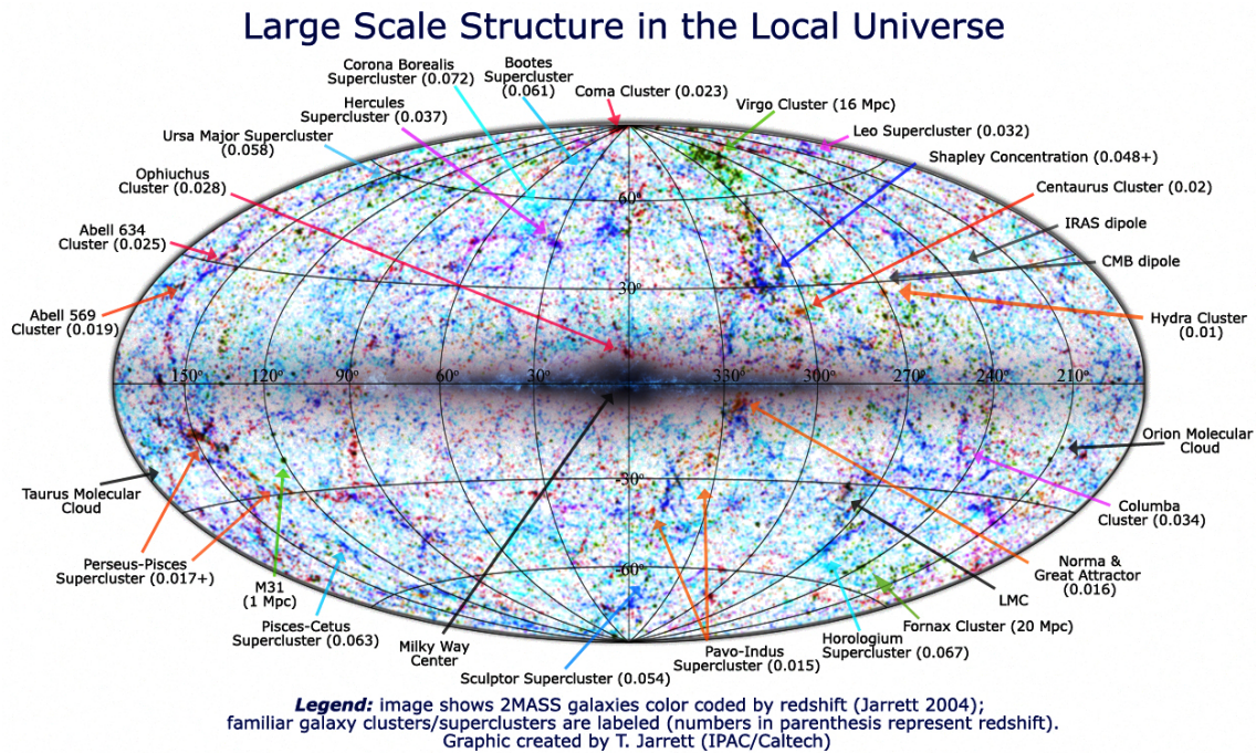
Figure 1.5: 2MASS image of our Milky Way and its surrounding environment, showing galaxies in the local group and the nearby large scale structure consisting of a range of galaxy clusters. Image courtesy: Tom Jarrett (IPAC/Caltech).
