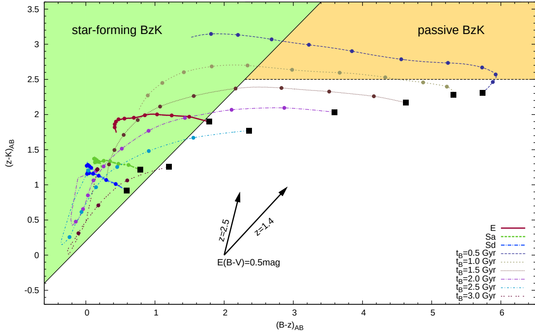
Figure 4.3: Colour selection scheme for BzK galaxies over-plotted with the part of our model grid that the BzK selection scheme aims at - galaxies with redshifts 1.4 \leq z \leq 2.5 . In the bottom middle of the plot we show reddening vectors for E(B - V) = 0.5\text{mag} for both extreme redshifts z = 1.4 and z = 2.5 . Large black squares mark the low-redshift end of the targeted redshift range at z = 1.4 . Thin lines mark the colour evolution of several models of Sb-progenitors undergoing a starburst with b_s = 0.75 at a galaxy age of t_B .
