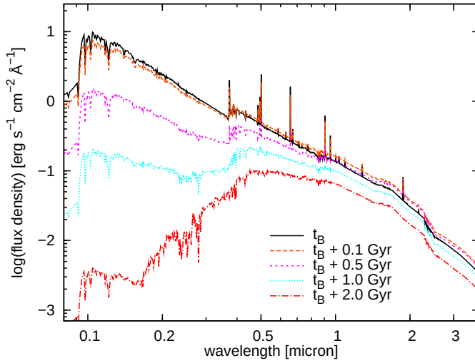
Figure 3.10: Spectra of a starburst galaxy, starting as a Sb-type model and encountering a strong (burst strength 75%) burst after 4 Gyr. Ages range from directly at the peak of the burst to late post-starburst phases.
