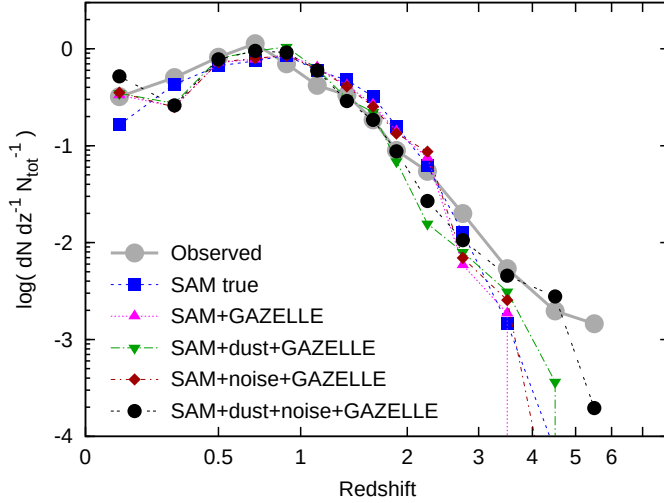
Figure 6.12: Comparison between the observed (thick grey line) projected density of galaxies per unit redshift, normalised by total number with the results from the artificial light-cones from Kitzbichler & White (2007) that are based on the Millennium simulation. The different lines represent results from different simulations also accounting for dust-extinction of photometric noise.
