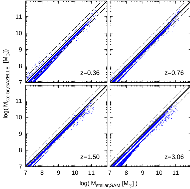
Figure 6.7: Comparison of stellar masses taken from the semi-analytical galaxy formation model of Bower et al. (2006) with the parameters obtained by fitting the synthetic rest-frame SEDs to a set of GALEV models using GAZELLE . Method and other details as in Fig. 6.6.
