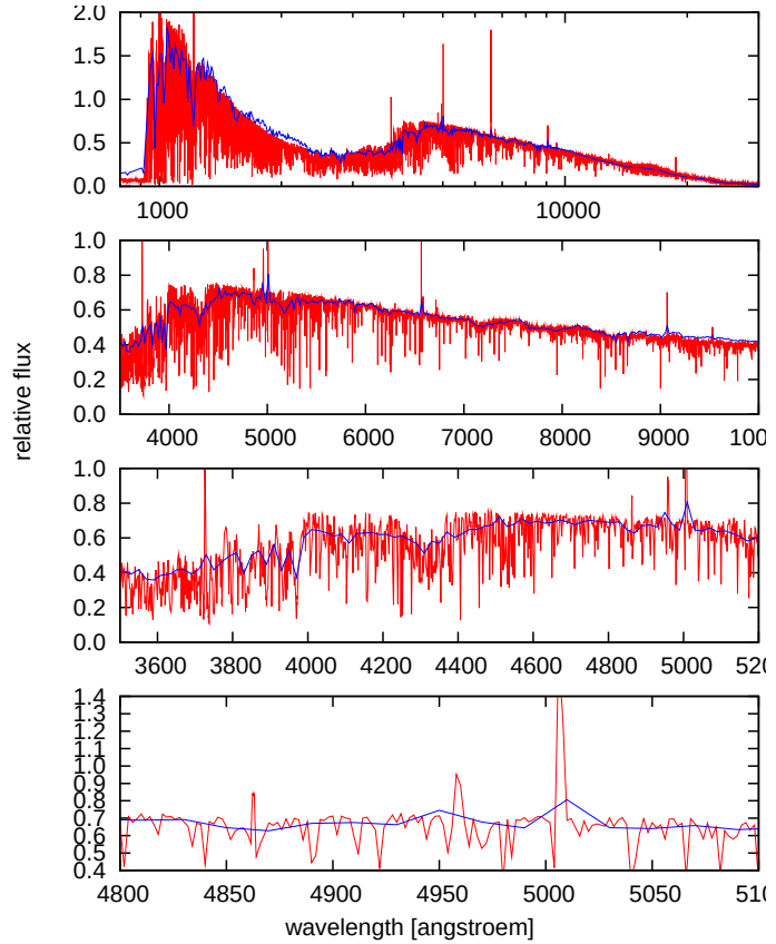
Figure 7.1: Illustration of a spectrum computed with the new intermediate-resolution library (red line, resolution 1\text{\AA} ), compared to a current low-resolution spectrum (blue line, wavelength resolution of 10\text{\AA} in the UV to 20\text{\AA} in the optical).
