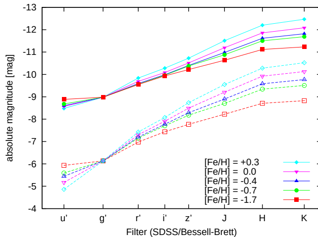
Figure A.1: Spectral energy distributions (SEDs) for star cluster models at two different ages of 1 Gyr at brighter and 13 Gyr at fainter absolute magnitudes, respectively, and 5 different metallicities ranging from 1/50 Z_{\odot} to 2.5 Z_{\odot} in each case. All SEDs have been scaled to match the g -band magnitude of the solar metallicity model with initial mass 10^6 M_{\odot} .
