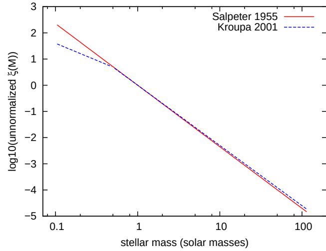
Figure C.2: Two examples of initial mass functions, here from Kroupa (2001) and Salpeter (1955)
