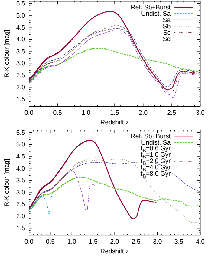
Figure 3.17: R - K colour evolution of models with bursts and remaining SF during the post-starburst phase for different progenitor types Sa to Sd (top panel) and different times of burst onset t_B = 0.6 - 8.0 Gyrs (bottom panel). The red solid line shows a model with Sb-type progenitor, a burst at a galaxy age of 2 Gyr and complete shutdown of SF after the burst as a reference with previous plots. The thick green line shows the colour evolution of our undisturbed Sa-type model.
