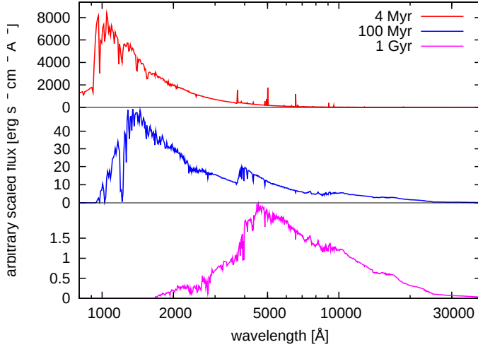
Figure C.7: Integrated isochrone spectra for the same isochrones shown in Fig. C.1 and Fig. C.5, including both stellar and gaseous emission.
