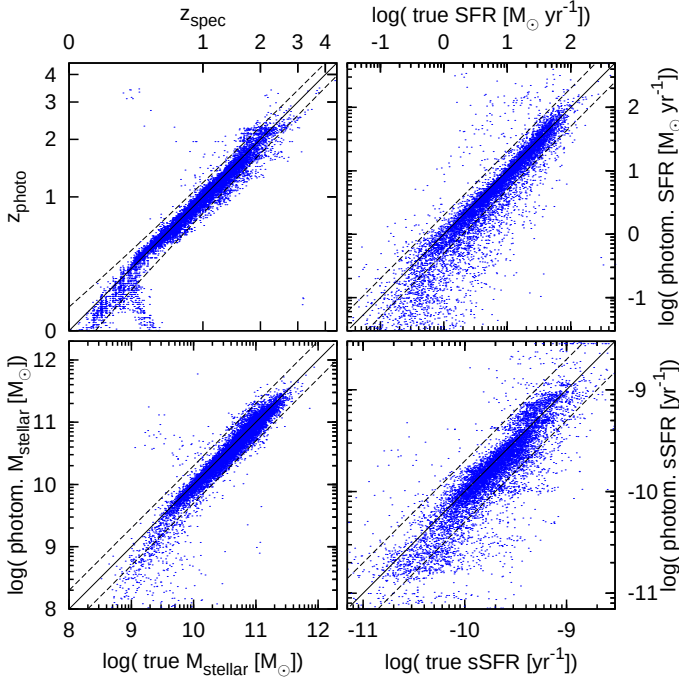
Figure 6.8: Comparison of redshifts and physical parameters obtained from fitting the simulated photometry with the true values as given by the semi-analytical models by Kitzbichler & White (2007) .
