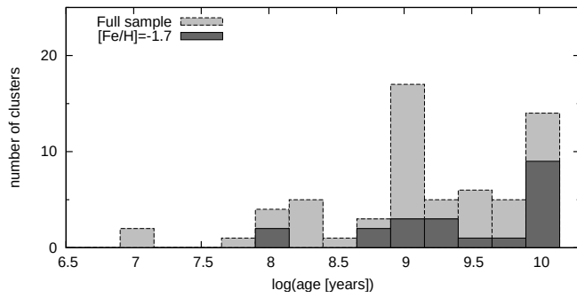
Figure A.4: Age distribution of our detected globular clusters.
