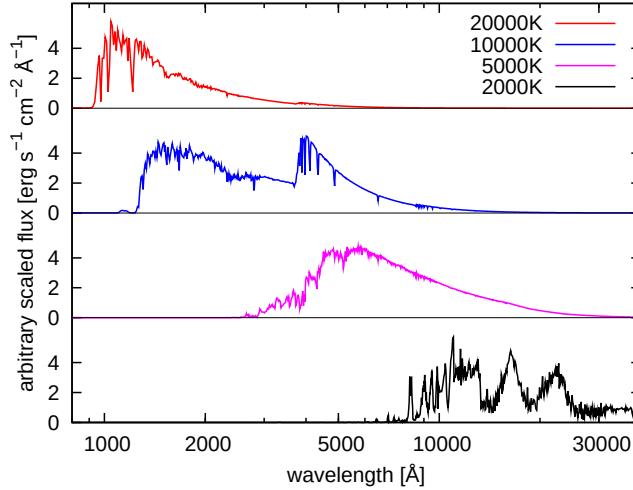
Figure C.4: Sample spectra from the Lejeune stellar library for stars with \log g = 4.0 and T_{\text{eff}} = (20000, 10000, 5000, 2000)\text{K} .
