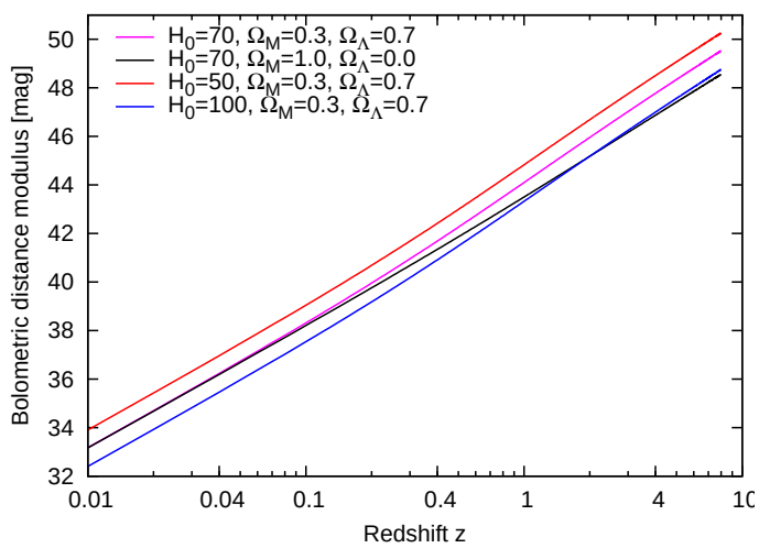
Figure C.16: Bolometric distance modulus as function of redshift for a range of cosmological parameter sets.
