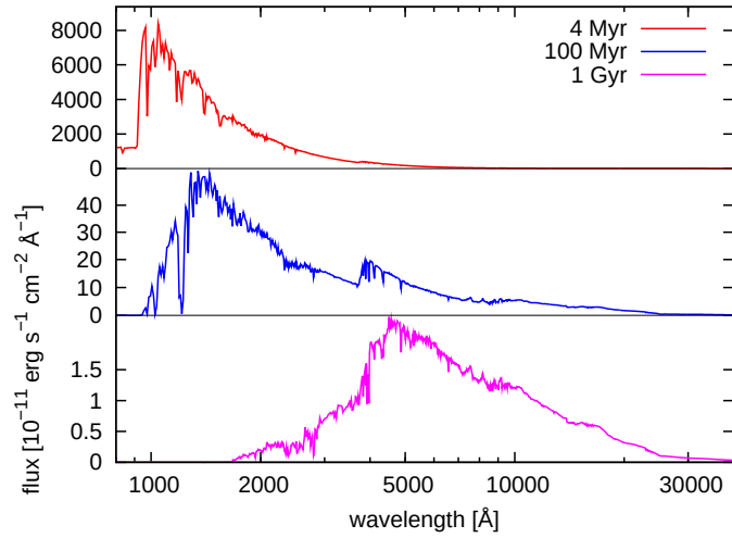
Figure C.5: Integrated starlight for the three isochrones shown in Fig. C.1.
