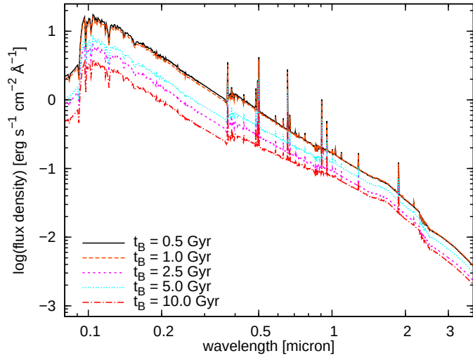
Figure 3.11: Comparison of spectra of burst models at the moment of maximum SFR for different onset times from 0.5 to 10 Gyr.
