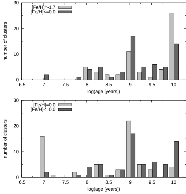
Figure A.9: Age distributions of our GC sample under the assumption of a fixed low metallicity [\text{Fe}/\text{H}] = -1.7 (upper panel) and [\text{Fe}/\text{H}] = 0.0 (lower panel). Bin sizes are the same as in Fig A.4, only the two histograms for free and restricted metallicities are plotted next to each other to better reveal the differences.
