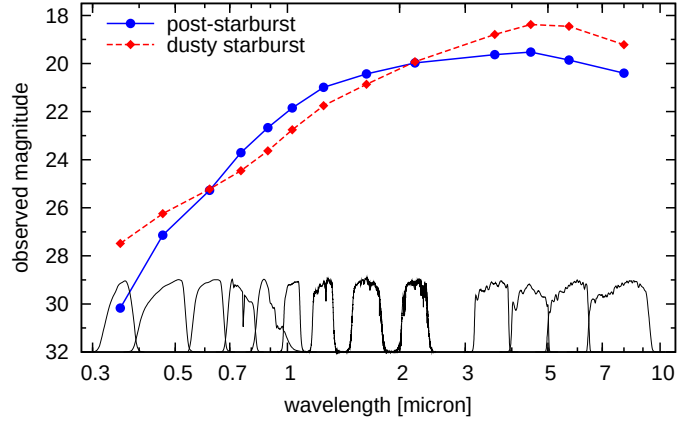
Figure 4.10: Comparison of a dusty starburst SED (red diamonds) and a post-starburst SED (blue circles) at redshift z = 1.6 , both having identical colours of r - K = 5.3 mag and normalized to K = 20 mag. The SED is formed by magnitudes in the SDSS ugriz, UKIDSS YJHK and IRAC [3.6],[4.5],[5.7] and [8.0] filters that are shown for reference on the bottom of the plot.
