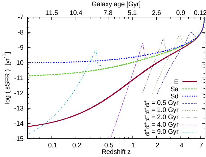
Figure 3.8: Specific star formation rates ( sSFRs, = SFRM_{\text{stellar}}^{-1} ) for a range of undisturbed models (thick lines) and starburst models (thinner lines). Starburst models are only shown for ages after the onset of the burst. The top axis gives the corresponding galaxy age.
