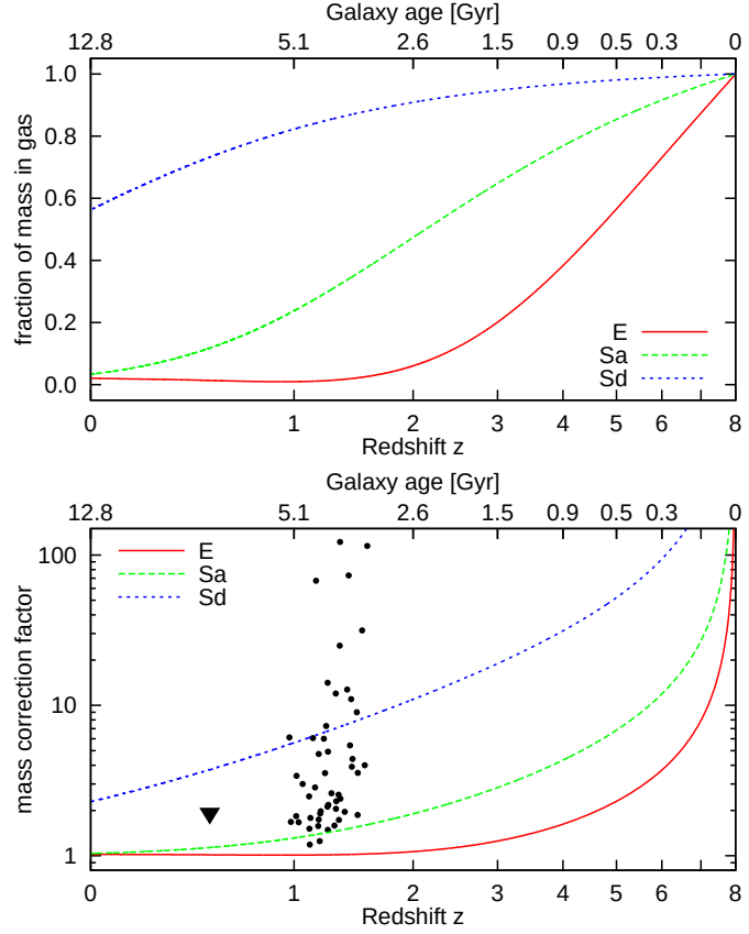
Figure 3.6: Top panel: Fractions of mass in gas relative to total mass for three different models as a function of redshift. Bottom panel: Photometric-to-dynamical mass correction factor for the same models shown in the top panel. The data points are observed data from Erb et al. (2006b) (small circles) and Daddi et al. (2008) (triangle). In both panels we give the corresponding galaxy age on the top axis.
