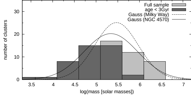
Figure A.7: Mass distribution of the GCs in NGC 4570. The light grey histogram is for all GCs from our sample, the dark one for the subsample of GCs younger than 3 Gyr. The solid line is a Gaussian fit to our unbinned GC mass distribution with a median of \log(\langle M_{GC}[M_\odot] \rangle) = 5.3 and \sigma(M_{GC}) = 0.6 dex, normalized to the number of GCs in our sample. The dotted line gives the Gaussian for the Milky Way GCs with \log(\langle M_{GC}[M_\odot] \rangle_{MW}) = 5.47 and \sigma_{MW}(M_{GC}) = 0.50 dex, normalized to the number of GCs in our sample.
