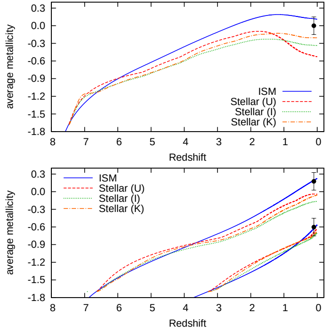
Figure 5.1: Chemical enrichment histories for galaxies of different spectral types E (top panel), Sa (lower panel, upper curves) and Sd (lower panel, lower curves). The blue solid lines marks the gas-phase or ISM-metallicity, while the dashed lines represent luminosity-weighted stellar metallicities in different bandpasses. Black points mark observed metallicities (Zaritsky et al., 1994) of local galaxies.
