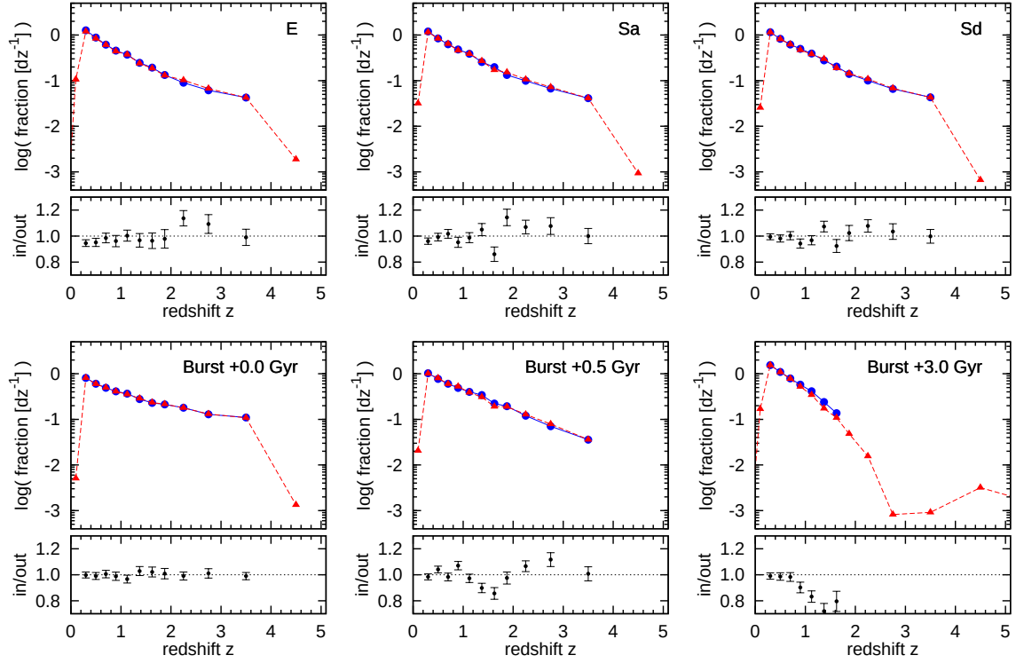
Figure 6.11: Results from our Monte-Carlo runs trying to explain the relative absence of galaxies in the redshift range z = 1.5 - 2 for six representative galaxy types (star formation histories) from our model grid. The top panels show, for each type, the input (blue circles) and the resulting redshift distribution after the photo-z fitting to the simulated photometry (red triangles). In the bottom panels we show the ratio between the number of galaxies in the output bin relative to the number of galaxies in the input catalog as a function of redshift. Error bars assume poissonian noise.
