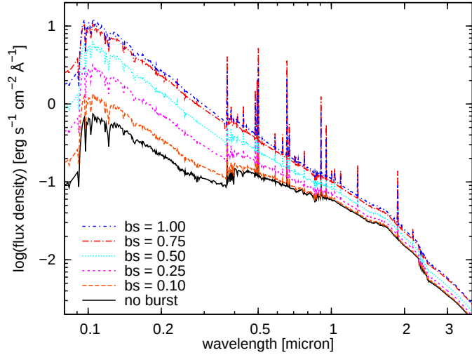
Figure 3.12: Comparison of spectra of burst models with identical onset times of 5 Gyr, but different burst strengths bs between 0.1 and 1.0.
