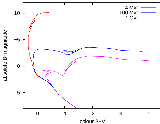
Figure C.1: Solar metallicity isochrones from the Padova group for three different ages of 4 Myr, 100 Myr and 1 Gyr
