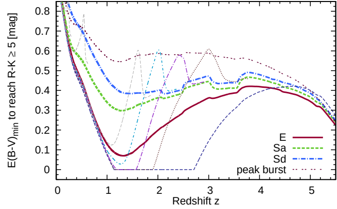
Figure 4.8: Minimum amount of dust reddening required to produce colours that reach the R - K > 5 \text{ mag} colour selection criterion. Several (post-)starburst are also shown but not included in the caption; for these the identification is identical with the one used in Fig. 4.6.
