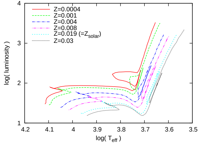
Figure 2.1: Stellar evolutionary tracks of a 2M_{\odot} star for different metallicities ranging between Z = 0.0004 = 1/50 Z_{\odot} and Z = 0.03 = 1.5 Z_{\odot} .
