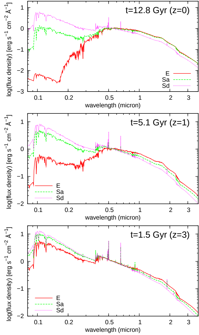
Figure 3.2: Comparison of spectra for three different spectral types E, Sa and Sd for three different ages of 12.8 Gyr (top panel), 5.1 Gyr (middle panel) and 1.5 Gyr (lower panel), corresponding to redshifts z=0 , z=1 and z=3 . All spectra are normalized to have unit flux at 0.55micron.
