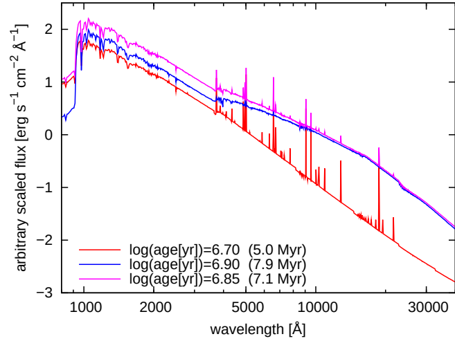
Figure C.8: Example for contributing isochrone spectra during interpolation in age.
