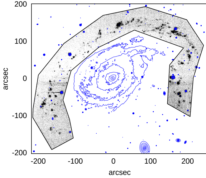
Figure B.2: Regions used to compute the SFR are shown in gray-scale with contour lines of the R-band image overplotted.
