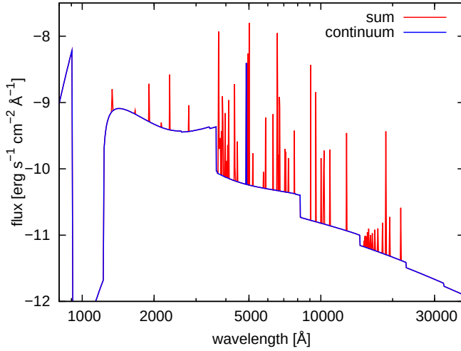
Figure C.6: Gaseous emission spectrum for solar metallicity. Shown in blue is the continuum emission, and continuum and line emission in red.
