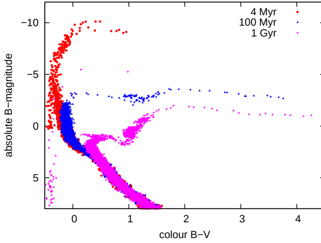
Figure C.3: Synthetic colour magnitude diagram where each point from the isochrone is assigned a numbers of stars based on the IMF. We added some scatter around each point to produce a smoother appearance.
