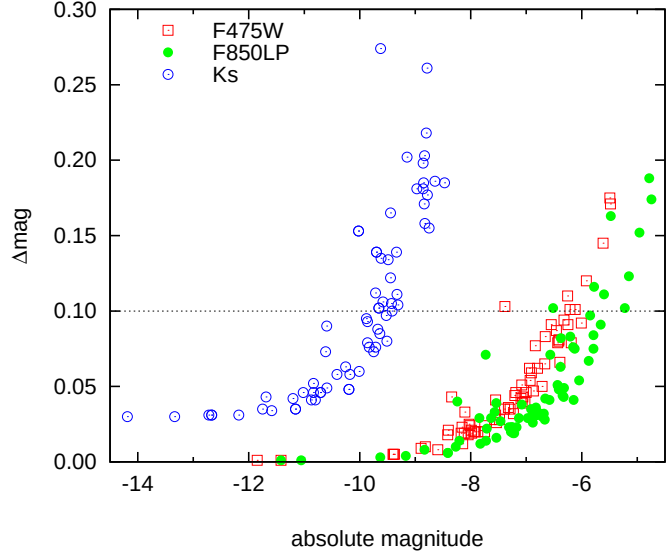
Figure A.2: Photometric errors as function of absolute magnitudes for the HST filters F475W and F850LP and the NTT filter K_s .
