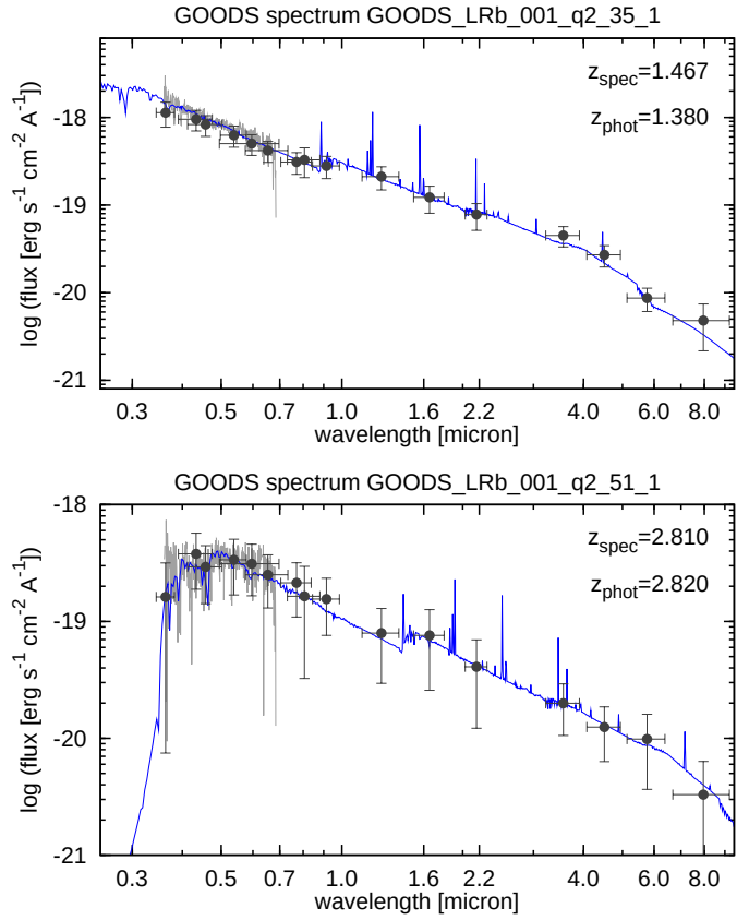
Figure 1.9: Examples of spectra for two galaxies at either side of the redshift range covered by the “redshift desert”. Observed spectra are shown as grey lines, observed photometric data-points and their respective uncertainties are shown with black circles; the blue solid line shows the best-fit spectrum obtained via the photometric redshift fitting.
