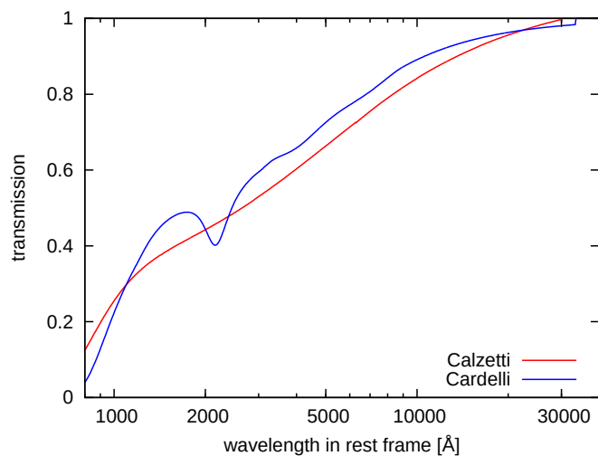
Figure C.12: Extinction curves from Calzetti and Cardelli. Both show very little transmission at short wavelengths indicating that most of the light gets absorbed.
