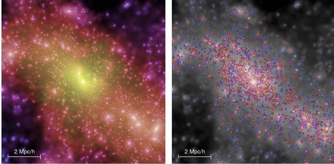
Figure 1.8: Comparison of the underlying dark matter distribution (left panel) and the visible galaxy population (right panel) inhabiting this distribution for one galaxy cluster in the Millennium simulation. The colours ranging from blue to red correspond to the stellar population age of the galaxy from young to old.
