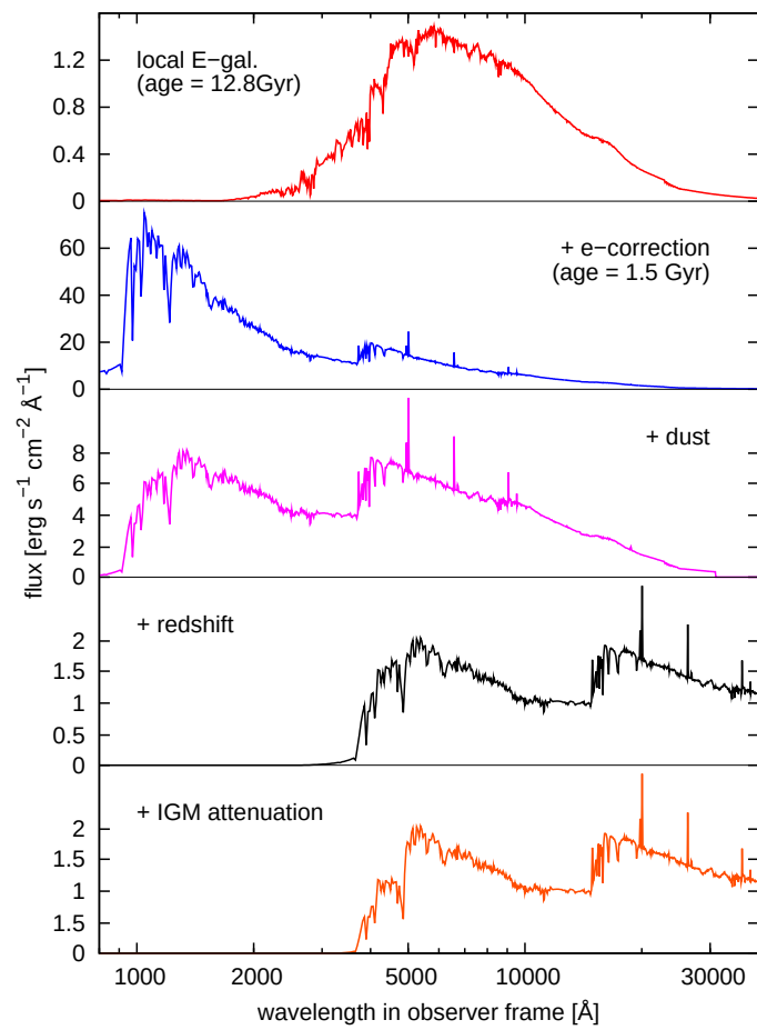
Figure C.14: Galaxy spectrum of an elliptical galaxy at different stages of the modelling process. Each following spectrum includes all effects shown above.
