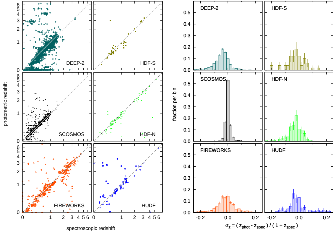
Figure 6.4: Comparison of spectroscopic and photometric redshifts.
