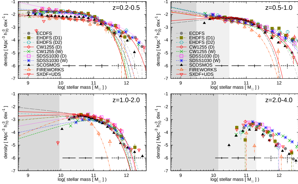
Figure 6.13: Mass functions for each of the fields in four different redshift bins (0.2, 0.5), (0.5, 1.0), (1.0, 2.0), and (2.0, 4.0). Points represent the actual data, while lines represent the best-fit Schechter functions. The grey-shaded regions mark the regions where incompleteness affects a) passive and predominantly old galaxies at the upper end of the redshift bin (light grey) and b) actively star-forming galaxies at the lower end of the redshift range (darker grey), both assuming no dust extinctions. Symbols in the lower panels are identical with those in the upper panels, but omitted to improve clarity. Small black error bars near the bottom of each panel indicate the additional uncertainty for each data-point as a result of cosmic variance, assuming a rectangular field size of 10 \times 10 arcmin, and using the recipe of Moster et al. (2010) .
