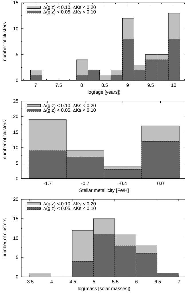
Figure A.8: Age, metallicity, and mass distributions for the subsample of GCs with high (light grey) and very high (dark grey) photometric accuracies.
