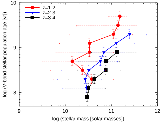
Figure 7.2: V-band light-weighted stellar population ages as function of stellar mass for three different redshift bins, based on data from the COSMOS survey. The effect of “downsizing” (more massive galaxies have older stellar populations than lower-mass galaxies) is nicely shown.
