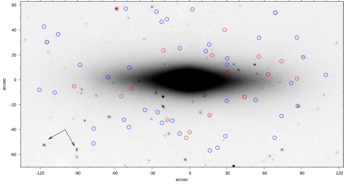
Figure A.5: Spatial distribution of our Globular Cluster sample, overlaid over our K-band image obtained with NTT/SOFI. Blue circles mark GCs with best-fit ages < 3 Gyr, while red circles mark GCs older than 3 Gyr. Most of the bright sources are either stars or (in most cases) background galaxies, that are resolved on the HST images.
