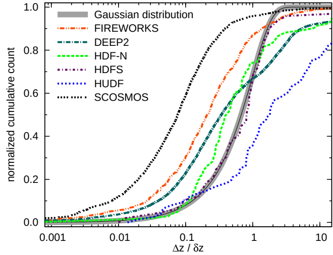
Figure 6.5: Cumulative distribution of \Delta z / \delta z (with \Delta z = |z_{\text{spec}} - z_{\text{phot}}| ; \delta z = (z_{\text{phot},+\sigma} - z_{\text{phot}}) for z_{\text{spec}} > z_{\text{phot}} and \delta z = (z_{\text{phot}} - z_{\text{phot},-\sigma}) for z_{\text{spec}} < z_{\text{phot}} ; z_{\text{phot},+\sigma} and z_{\text{phot},-\sigma} are the upper and lower 1\sigma extremities, respectively) for all galaxies in our sample with available spectroscopic redshift. For comparison we show the expected distribution in case of gaussian errors.
