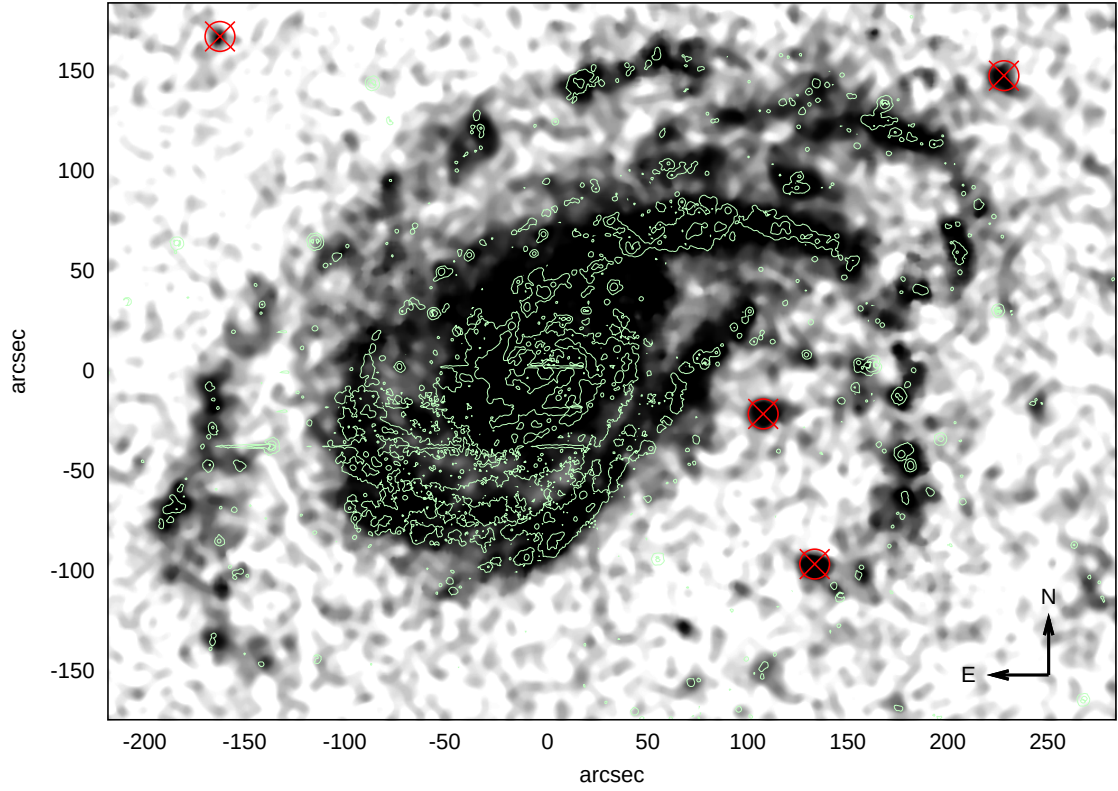
Figure B.1: The far-UV image of Arp 78 shown as gray-scales is overplotted with contour lines for the H\alpha emission. The four circles mark positions of three background galaxies and a point source (probably an AGN or a hot star) that show up in the FUV, but not in our H\alpha images.
