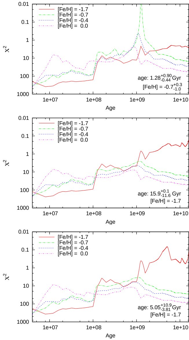
Figure A.3: \chi^2 values as function of metallicity and age for 3 different clusters.
