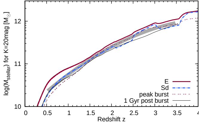
Figure 4.9: Minimum stellar mass that is required to reach an apparent magnitude of K = 20 mag. The grey thick line shows a 2nd-order polynomial fit to the models (see text for parameters).
