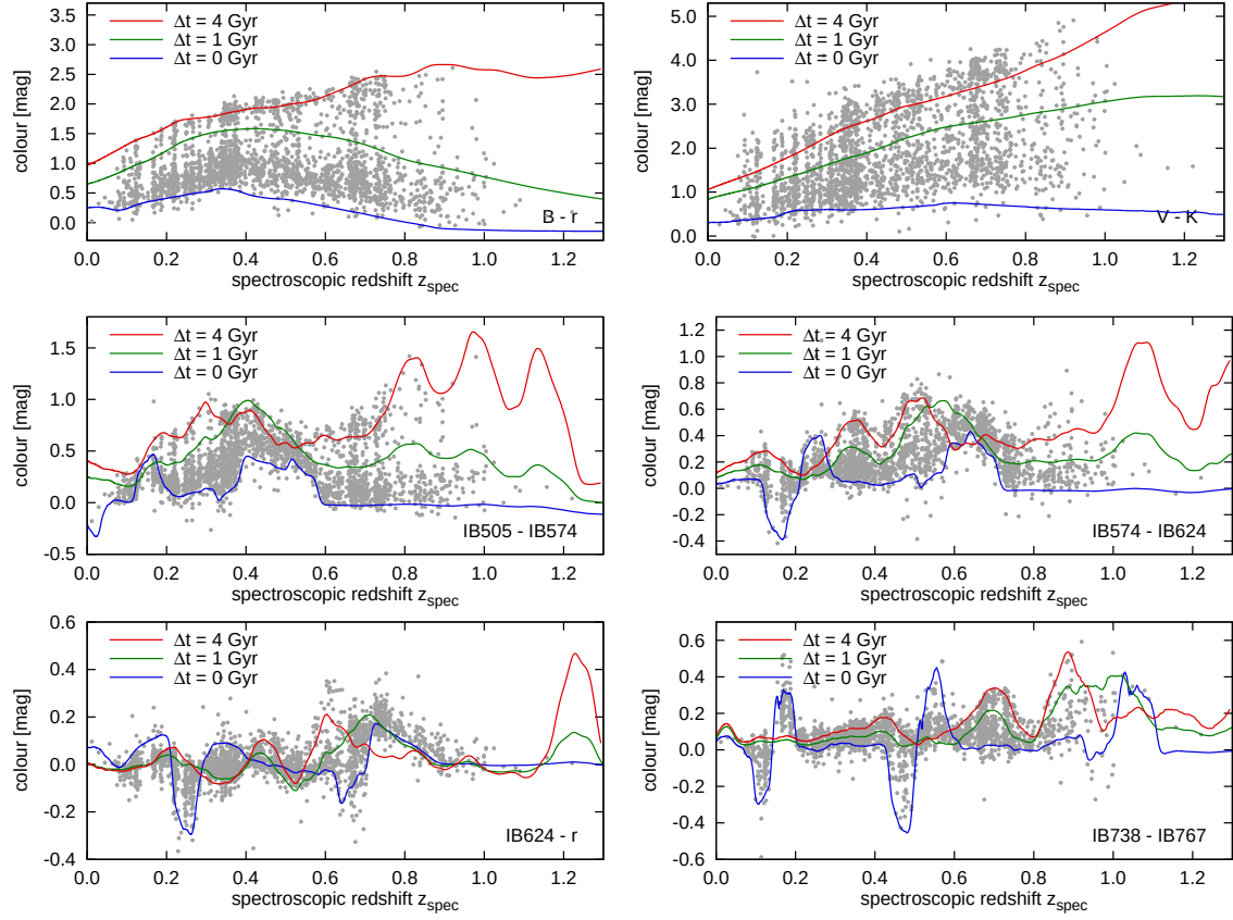
Figure 6.2: Comparison of the colour evolution with spectroscopic redshift as observed in COSMOS for a range of filter combinations (observed colours shown with grey dots): Top row: B - r (left), V - K (right); middle row: IB505 – IB574, IB574 – IB624; bottom row: IB624 – r , IB738 – IB767. For comparison we show three of the models in our grid, a starburst at peak SFR ( \Delta t = 0 ) and two post-starburst models \Delta t = 1 Gyr and \Delta t = 4 Gyr after the SFR peak, each using a metallicity of 0.5 Z_{\odot} .
