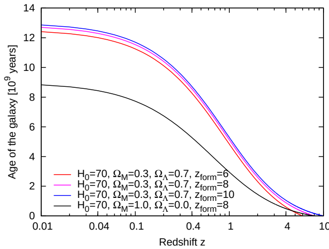
Figure C.11: Relation between galaxy age and redshift for different cosmological parameters and in particular varying formation redshifts.
