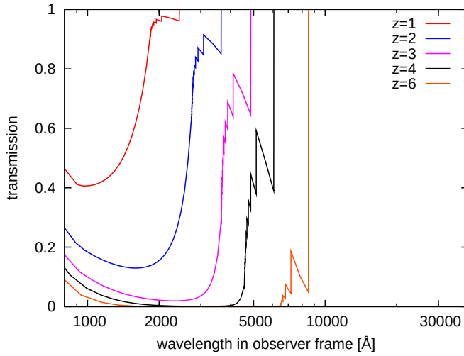
Figure C.13: Transmission of the intergalactic medium as function of observed frame wavelength for sources at different redshifts.
