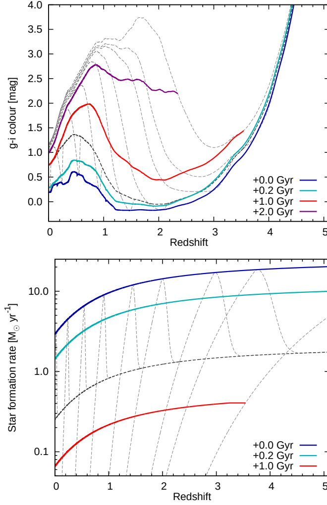
Figure 2.9: Comparison between several “traditional” models and several derived “iso-evolution” models, shown as coloured lines in blue, cyan, red and violet, corresponding to burst-ages of 0.0 (at the peak of SFR), 0.2, 1.0, and 2.0 Gyr. Dashed grey lines mark the traditional models for burst onset times ranging from 0.12 to 12.5 Gyr. The darker dashed line shows the evolution of the underlying, undisturbed Sb-type model.
