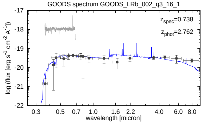
Figure 1.11: Same as Fig. 1.9, but for a case with discordant spectroscopic and photometric redshifts. For the observed spectrum, the redshift is supposedly based on the detection of the \text{Mg II } \lambda 2798 and [\text{O II}] \lambda 3727 lines.
